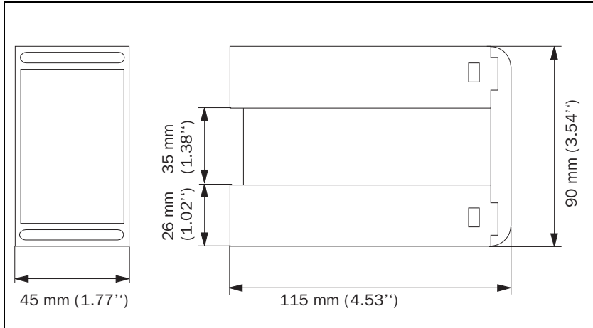
Fig. 17 DCM dimensions
