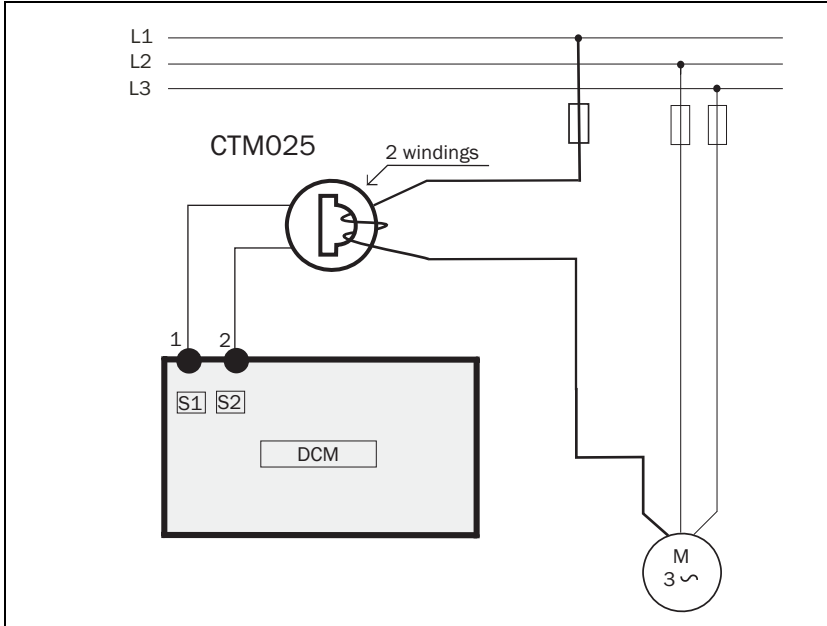
Fig. 6 Example: CTM 025 with 2 windings for a 12 A pump motor
