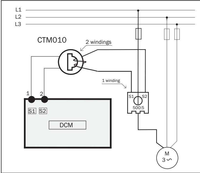
Fig. 8 Example of a CTM 010 with 2 windings and a primary transformer 500:5 with 1 winding for a 260 A pump motor. See also note on page 15
