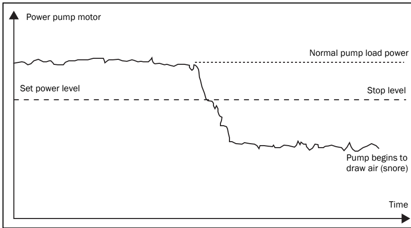
Fig. 1 Pump operation
