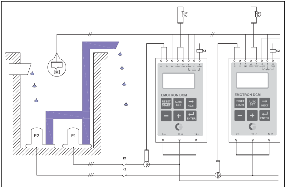
Fig. 15 Dual-pump application
